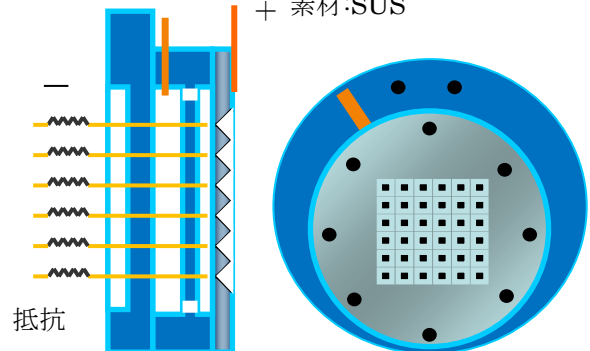
Fig.2 Isolation of each electrode array thruster.
