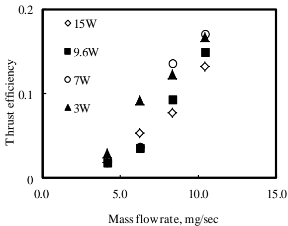
Fig.9 Thrust efficiency vs mass flow rate for comparison of nozzle performance.
