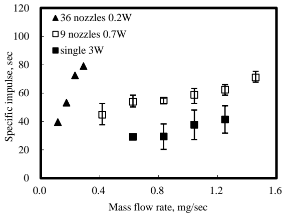
Fig.11 Specific impulse vs mass flow rate for comparison of nozzle performance.
